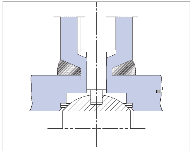
WELDED EXTENSION - DETAIL
