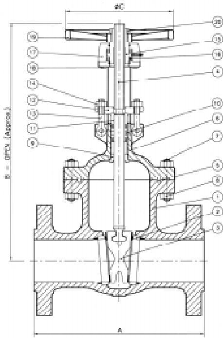
FLANGED END
