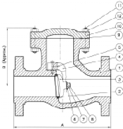
FLANGED END
