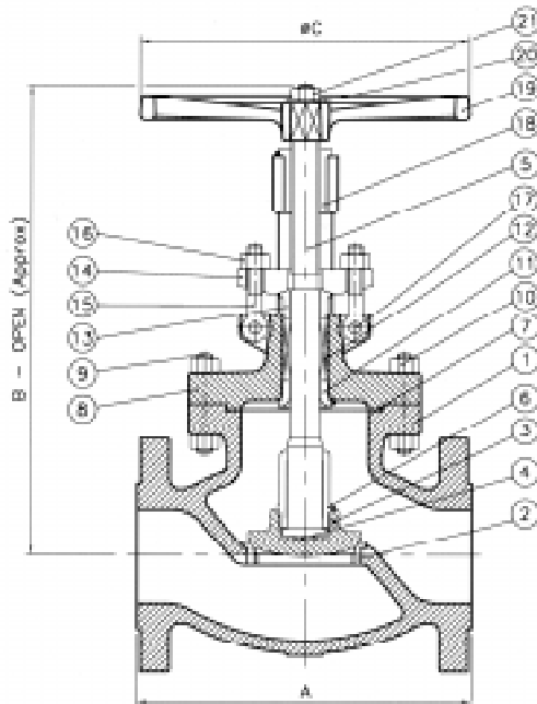
FLANGED END
