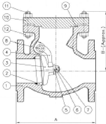
FLANGED END
