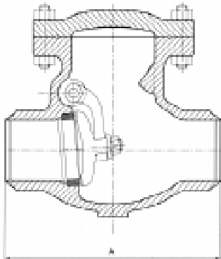
BUTT-WELD END
