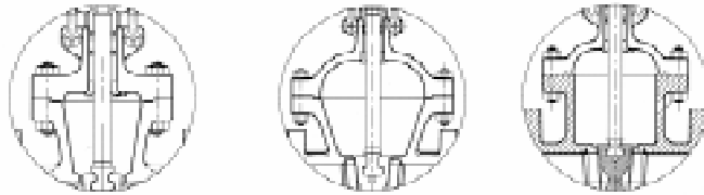
BUTT-WELD END
