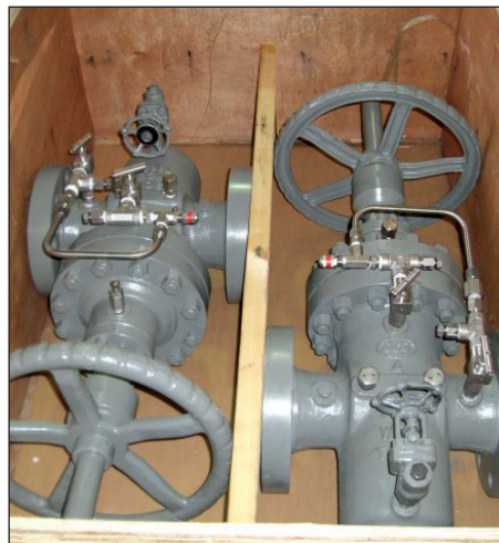
SCV installed Thermal Relief system on 4" Class 600 Thru Conduit Gate Valves
